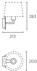
05-3217-19-82 + PAN-157-BY
