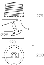
05-2756-81-21 + PAN-219-14
