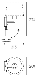
05-3218-21-82 + PAN-157-14
