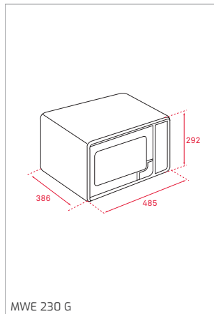
MWE 230 G
