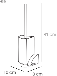
10607 Escobillero Brush holder Porte-brosse
