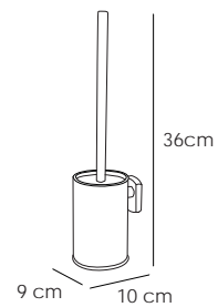
11977 Escobillero Cromo 43 € Brush holder Porte-brosse
