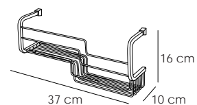
60019 Jabonera rejilla JR-19 Cromo 70 € Soap grid JR-19 Savon grille JR - 19
