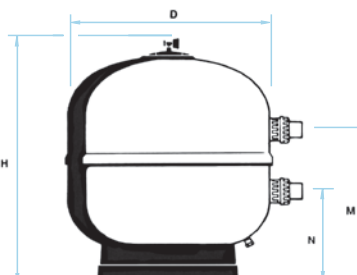
Filtro sin válvula Without valve filter
